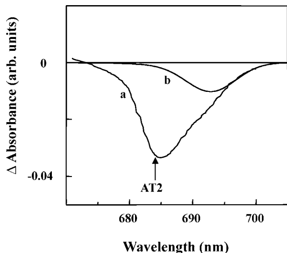
Figure 11. Curve a corresponds to the SADS spectrum of CP47 adopted from Figure 7 in ref 19, which was obtained on a few ns time scale. Curve b (expanded to fit the lowest-energy tail of spectrum a) is the A1 band from Figure 7B (this work). The upward arrow below curve (a) indicate possible contribution to the SADS spectrum from the AT2 trap.
